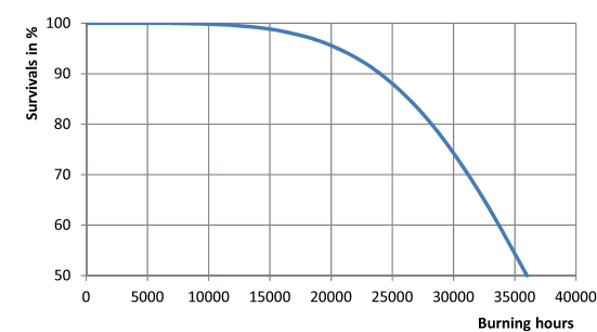
Life Expectancy Diagram - MST SON-T PIA Plus 400W E40 1SL/12
