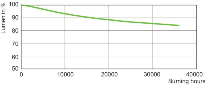
Lumen Maintenance Diagram - MST SON-T PIA Plus 400W E40 1SL/12
