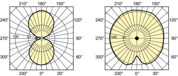
Light Distribution Diagram - MST SON-T PIA Plus 400W E40 1SL/12
