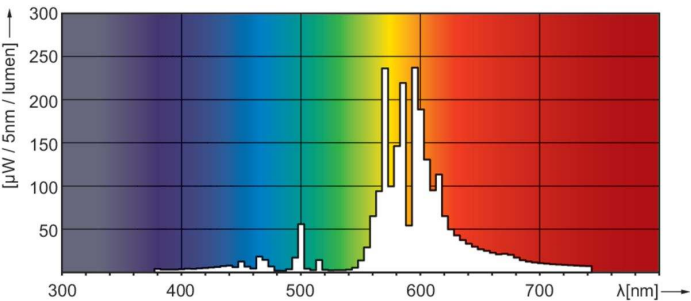
Spectral Power Distribution Colour - MST SON-T PIA Plus 400W E40 1SL/12
