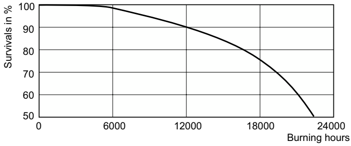
Life Expectancy Diagram - MASTER SOX-E 18W BY22d 1SL/12
