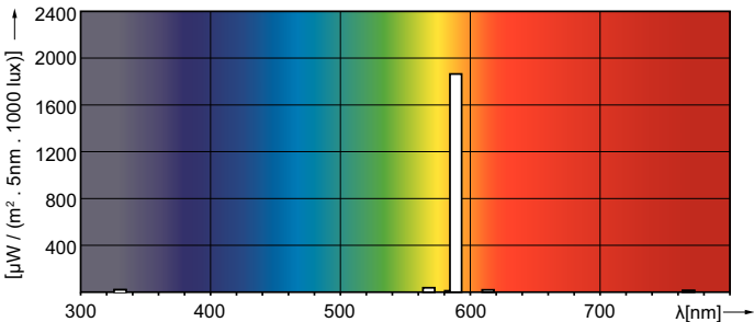
Spectral Power Distribution Colour - MASTER SOX-E 36W BY22d 1SL/12
