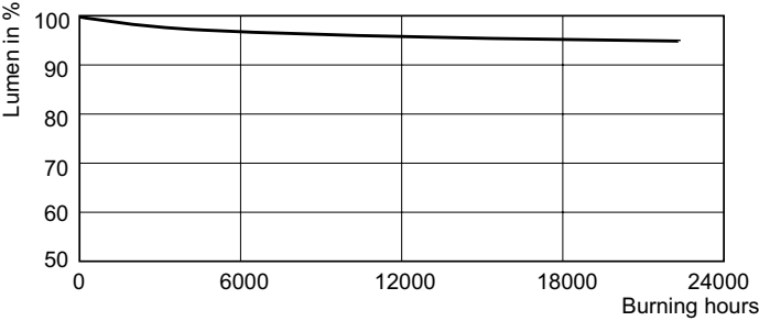
Lumen Maintenance Diagram - SOX 180W BY22d 1SL/6
