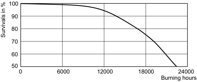
Life Expectancy Diagram - MASTER SOX-E PSG 36W BY22d T50 1SL/12
