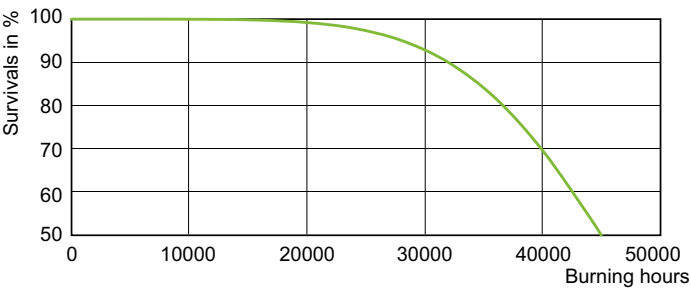
Life Expectancy Diagram - MST SON-T APIA Plus Xtra 250W E40 1SL/12
