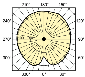
Light Distribution Diagram - MST SON-T APIA Plus Xtra 250W E40 1SL/12
