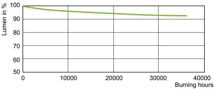
Lumen Maintenance Diagram - MST SON-T PIA Plus 150W/220 E40 - 1SL/12
