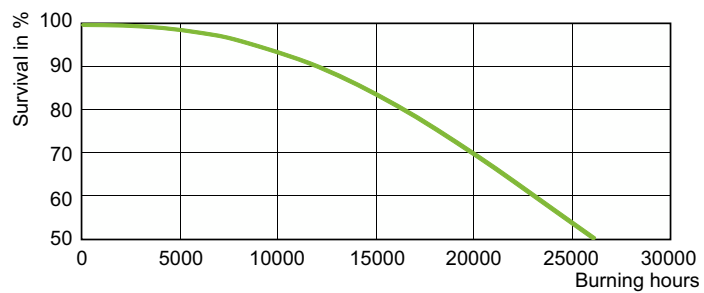
Life Expectancy Diagram - SON H 220W/220 E40 1SL/12
