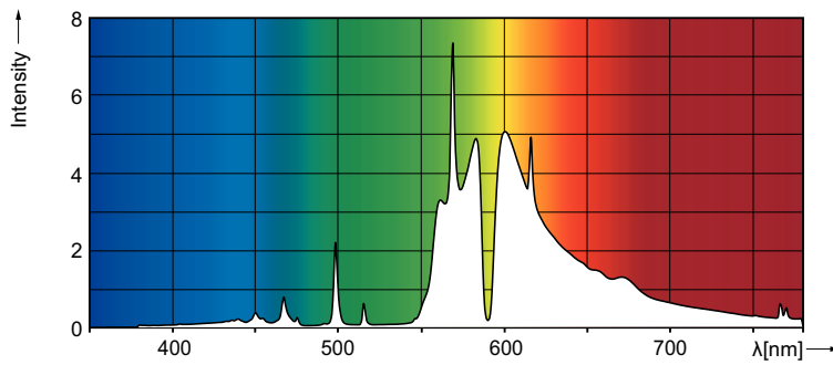
Spectral Power Distribution Colour - MASTER GreenPower Xtra 1000W EL/5X6CT
