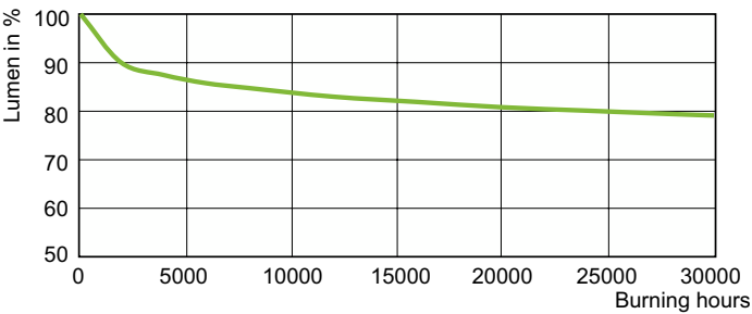
Lumen Maintenance Diagram - MST SON-T PIA Plus 70W E E27
