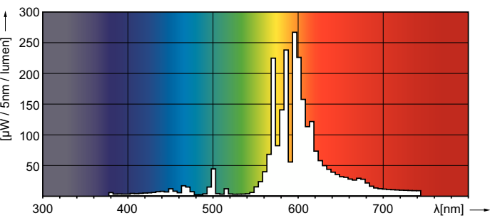
Spectral Power Distribution Colour - MST SON-T PIA Plus 70W E E27
