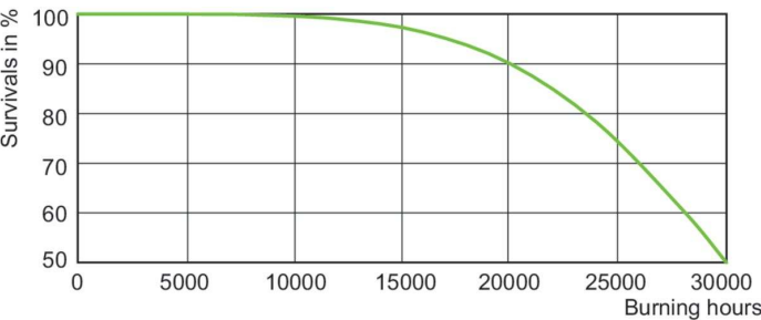
Life Expectancy Diagram - MST SON-T PIA Plus 70W E E27
