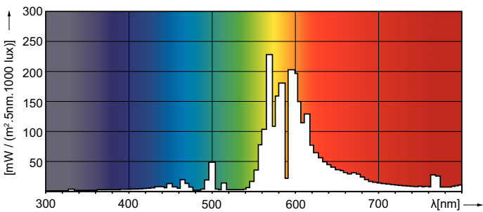
Spectral Power Distribution Colour - MASTER SON PIA Plus 250W/220 E40 1SL/12
