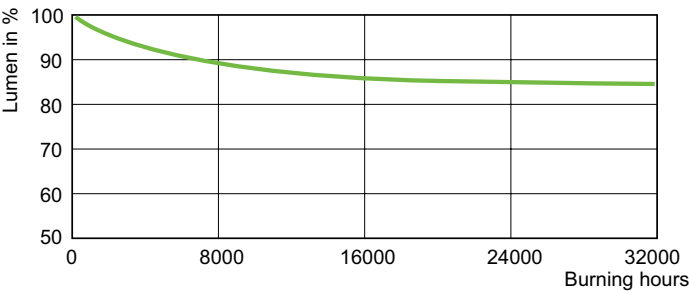
Lumen Maintenance Diagram - MASTER GreenPower CG T 600W E40
