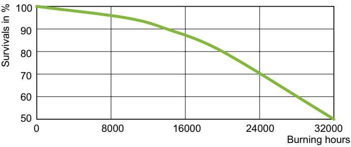
Life Expectancy Diagram - MASTER GreenPower CG T 600W E40
