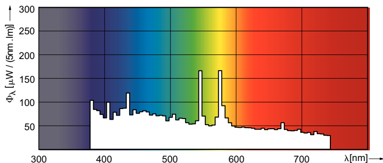
Spectral Power Distribution Colour - MSR Gold 1200 SA/2 DE UNP/108
