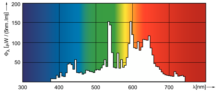
Spectral Power Distribution Colour - MASTERC CDM-T Elite 70W/930 G12 1CT/12
