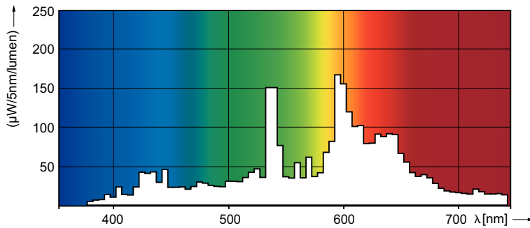
Spectral Power Distribution Colour - MASTERColour CDM-TC Elite 50W/930 G8.5 1CT/12
