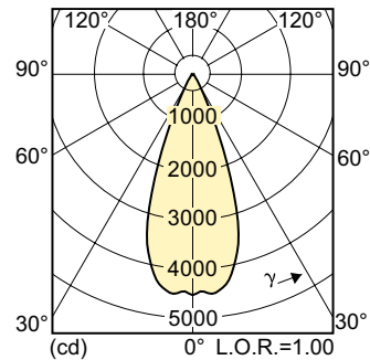
Light Distribution Diagram - MASTERC CDM-R111 Elite 35W/930 GX8.5 40D
