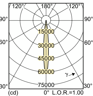
Light Distribution Diagram - MASTERC CDM-R111 Elite 70W/930 GX8.5 10D
