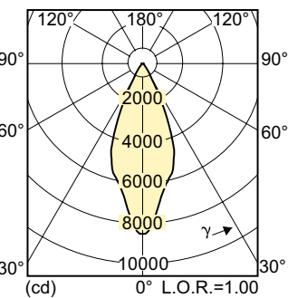
Light Distribution Diagram - MASTERC CDM-R111 Elite 70W/930 GX8.5 40D
