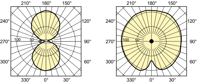
Light Distribution Diagram - MST SON-T APIA Plus Hg Free 70W E27 1SL
