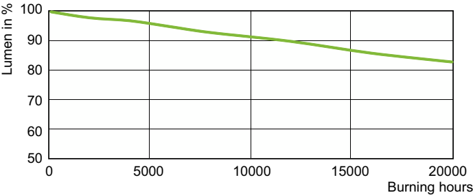
Lumen Maintenance Diagram - MST SON-T APIA Plus Hg Free 70W E27 1SL
