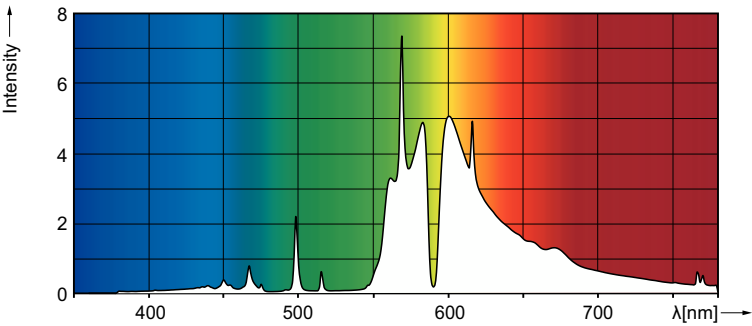
Spectral Power Distribution Colour - HPS AGRO Plus 1000W DE EL 1CT/12
