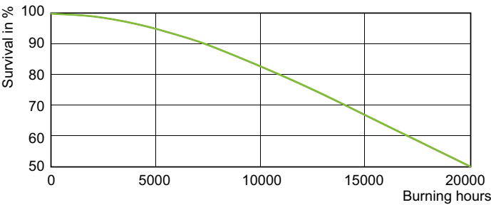
Life Expectancy Diagram - MASTER HPI-T Plus 400W/643 CL 1SL
