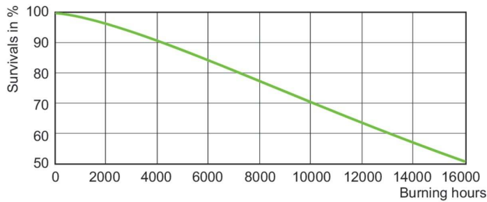
Life Expectancy Diagram - MH Quartz 400W/637 E40 CO U 1SL/6
