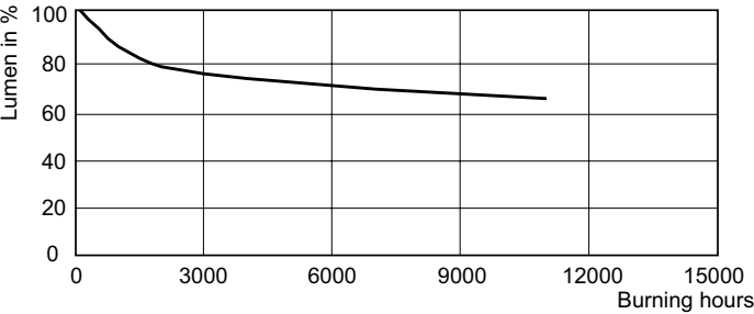
Lumen Maintenance Diagram - MHN-TD Essential 70W/742 RX7s 1CT/12
