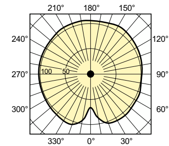
Light Distribution Diagram - SON-T 100W E E40 SL/12
