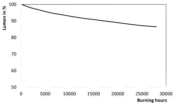
Lumen Maintenance Diagram - MST SON-T PIA Plus 100W E E40
