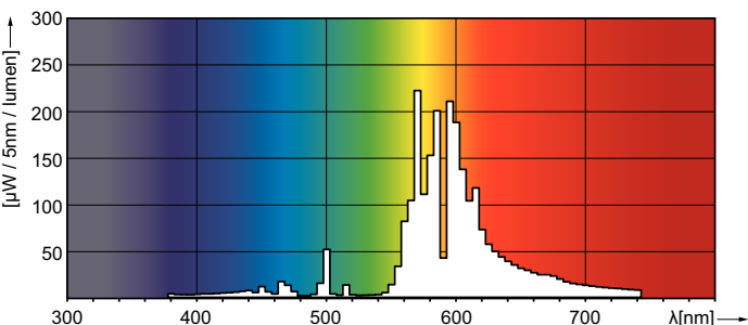
Spectral Power Distribution Colour - MST SON-T PIA Plus 150W E E40
