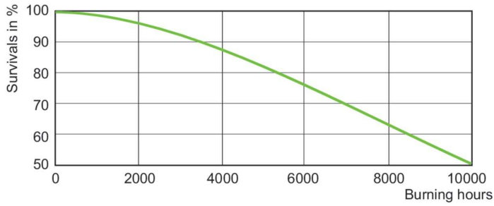
Life Expectancy Diagram - MH 150W/640 E27 CL 1SL/24
