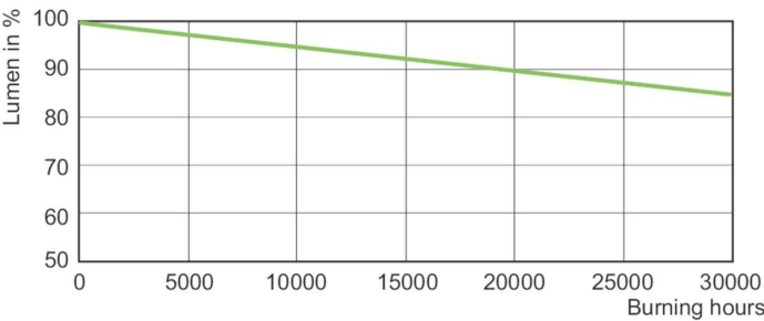
Lumen Maintenance Diagram - SON-T 150W E E40 1SL/12
