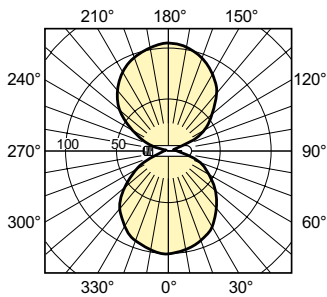
Light Distribution Diagram - SON-T 150W E E40 SL/12
