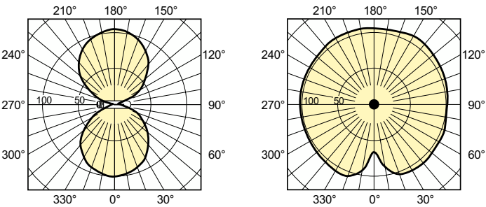
Light Distribution Diagram - SON-T 250W E E40 1SL
