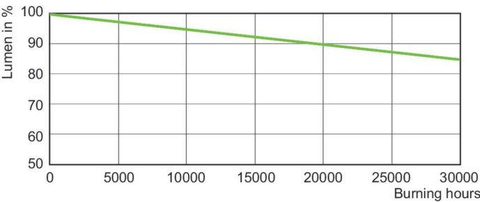
Lumen Maintenance Diagram - SON-T 250W E E40 1SL
