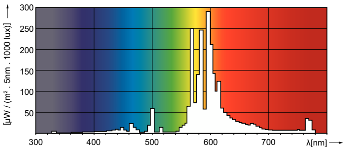
Spectral Power Distribution Colour - SON-T 250W E E40 1SL
