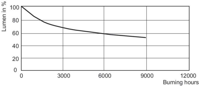
Lumen Maintenance Diagram - MASTERC CDM-R 35W/830 E27 PAR30L 10D 1CT
