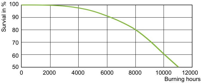
Life Expectancy Diagram - MASTERC CDM-R 35W/830 E27 PAR30L 10D 1CT
