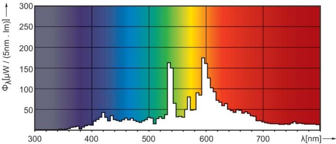
Spectral Power Distribution Colour - MASTERC CDM-R 35W/830 E27 PAR30L 10D 1CT
