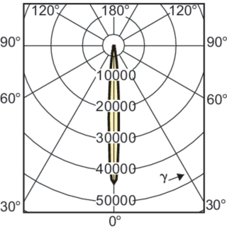
Light Distribution Diagram - MASTERC CDM-R 35W/830 E27 PAR30L 10D 1CT
