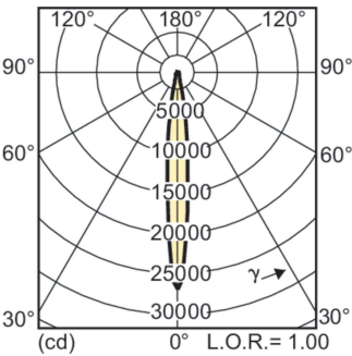
Light Distribution Diagram - MASTERC CDM-R 35W/942 E27 PAR20 10D 1CT
