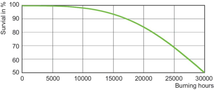
Life Expectancy Diagram - SON 100W E E40 CO 1SL
