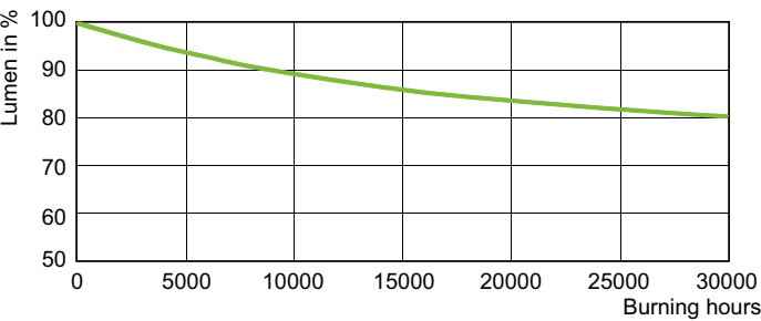
Lumen Maintenance Diagram - SON 100W E E40 CO 1SL
