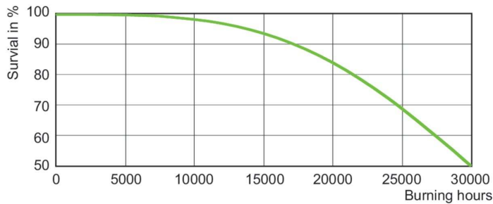
Life Expectancy Diagram - SON 100W E E40 CO 1SL
