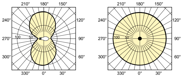
Light Distribution Diagram - SON 100W E E40 CO 1SL
