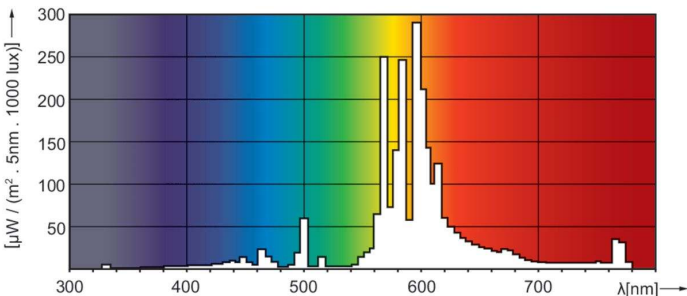
Spectral Power Distribution Colour - SON 100W E E40 CO 1SL
