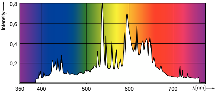
Spectral Power Distribution Colour - CDM ELITE MW 210/930/U/O
