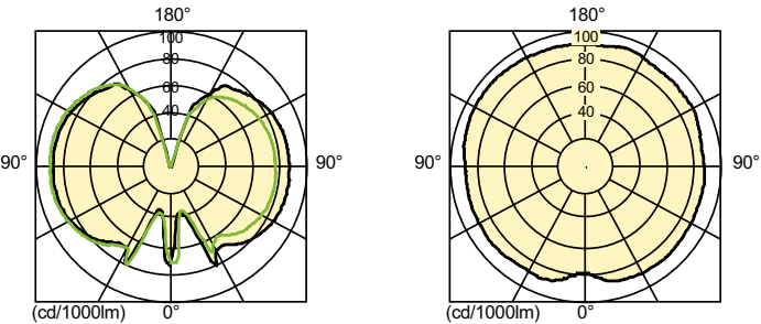
Light Distribution Diagram - CDM ELITE MW 210/930/U/O
