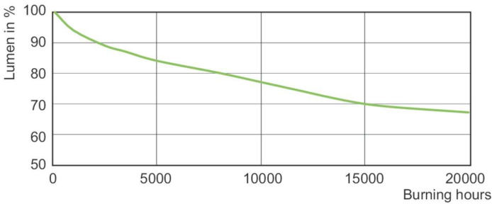
Lumen Maintenance Diagram - CDM145/U/O/4K/ED28 EA ALLSTART
