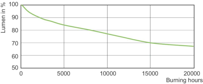
Lumen Maintenance Diagram - CDM145/U/4K/ED17 EA Allstart
