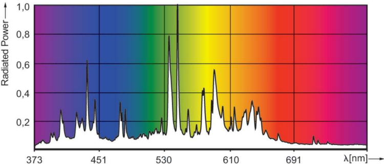
Spectral Power Distribution Colour - CDM145/U/4K/ED17 EA Allstart
