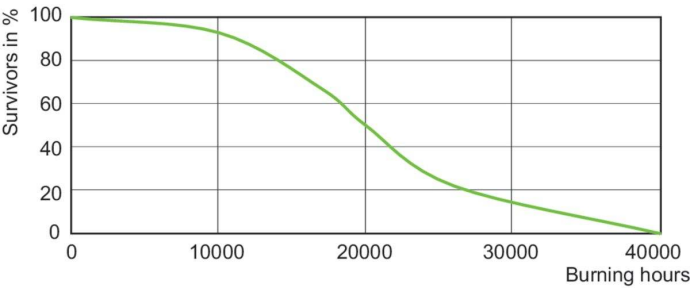
Life Expectancy Diagram - CDM145/U/4K/ED17 EA Allstart
