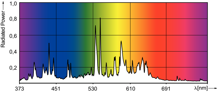
Spectral Power Distribution Colour - CDM145/C/U/O/4K/ED28 EA Allstart
