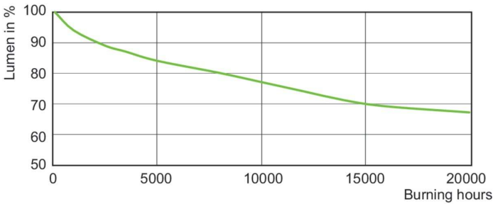
Lumen Maintenance Diagram - CDM145/C/U/O/4K/ED28 EA Allstart
