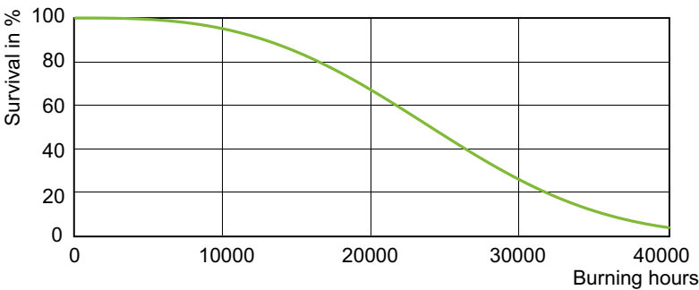
Life Expectancy Diagram - MHC150/U/M/3K ALTO 12PK
