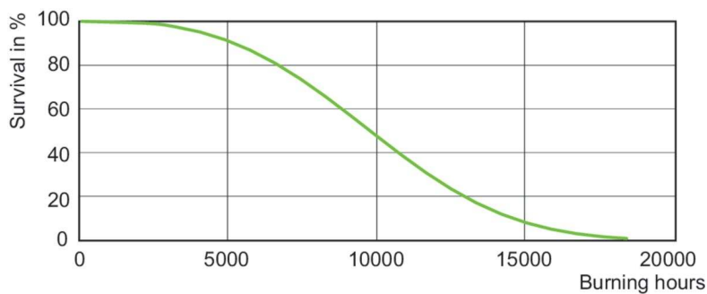
Life Expectancy Diagram - MHC100/C/U/M 3K ELITE
