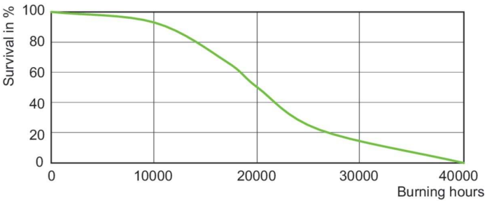
Life Expectancy Diagram - CDM 210/U/O/4K ED28 12PK
