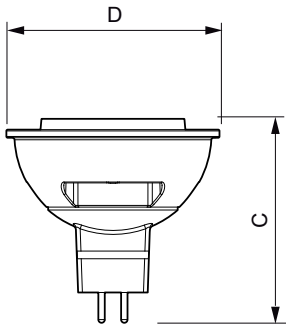
LED 4-20W GU5.3 830 MR16 24D
