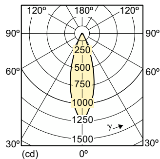
Light Distribution Diagram - MASTER LED 7-50W 2700K MR16 36D Dim
