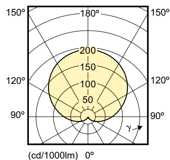
Light Distribution Diagram - CorePro LEDbulb 4-32W E27 830
