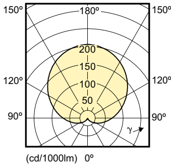
Light Distribution Diagram - CorePro LEDbulb 9-60W E27 830
