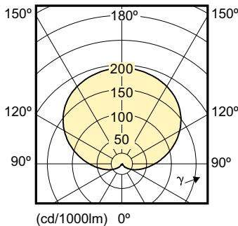
Light Distribution Diagram - CorePro LEDbulb 10.5-75W E27 830
