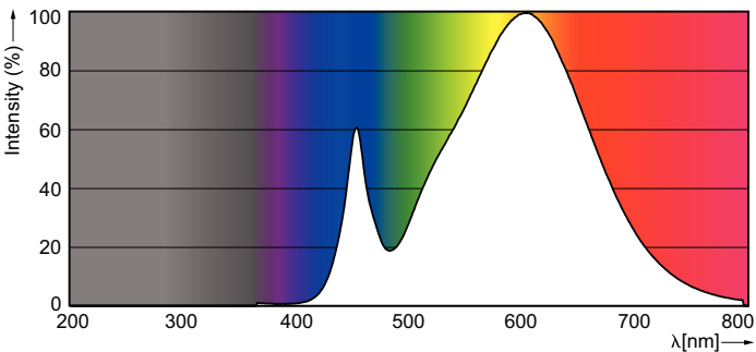
Spectral Power Distribution Colour - CorePro LEDbulb 10.5-75W E27 830
