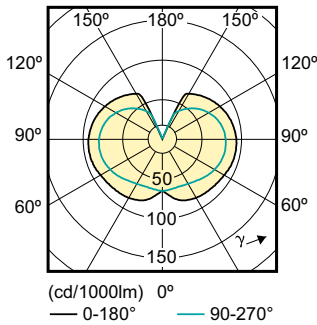
Light Distribution Diagram - SlimStyle A19 10.5W E26 2700K 120V ES
