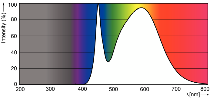
Spectral Power Distribution Colour - MAS LEDtube 1500mm SO 20W 840 T8
